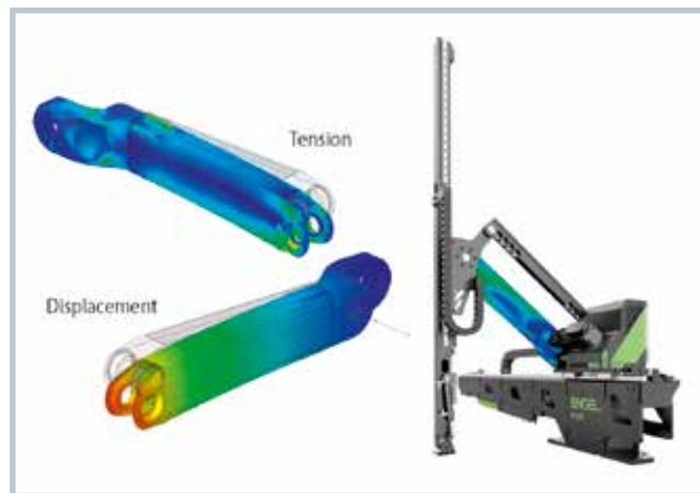
Fig. 3. The rotational axis was designed with an assembled profile of carbon tapes and a stub of die-cast aluminum for connecting to the servo motor (© Engel)
